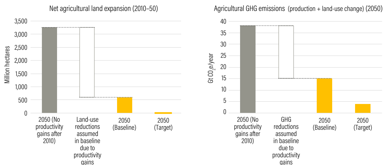
Figure 9 | Improvements in crop and livestock productivity already built into the 2050 baseline close most of the land and GHG mitigation gaps that would otherwise exist without any productivity gains after 2010
