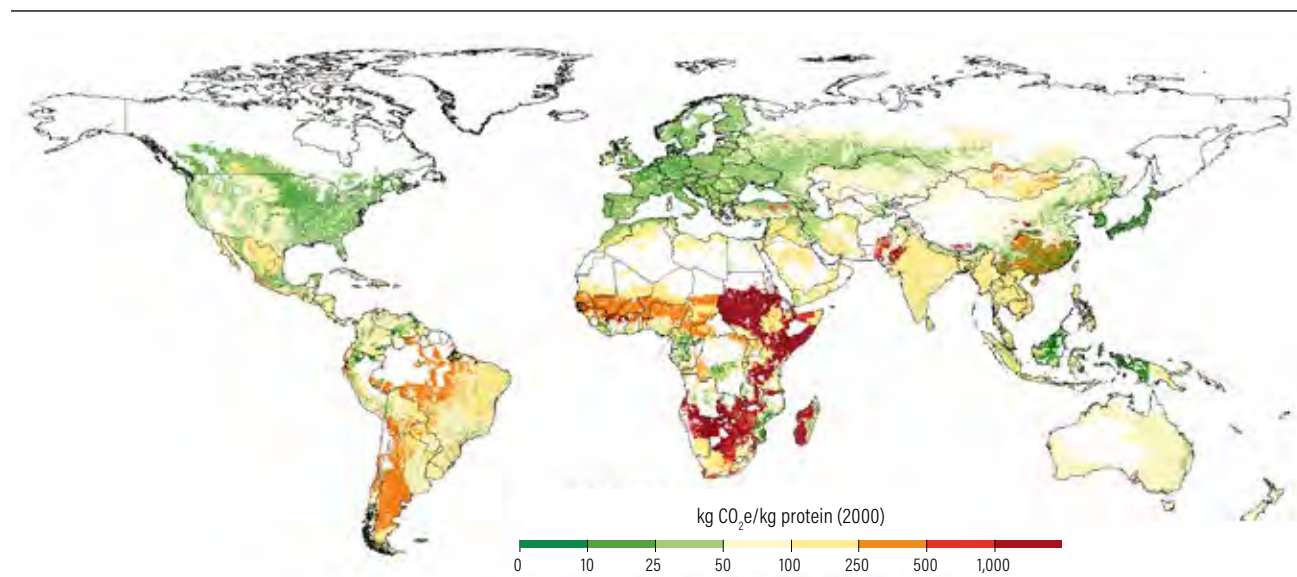
Figure 10 | Inefficient beef production systems result in far higher greenhouse gas emissions per unit of meat output
