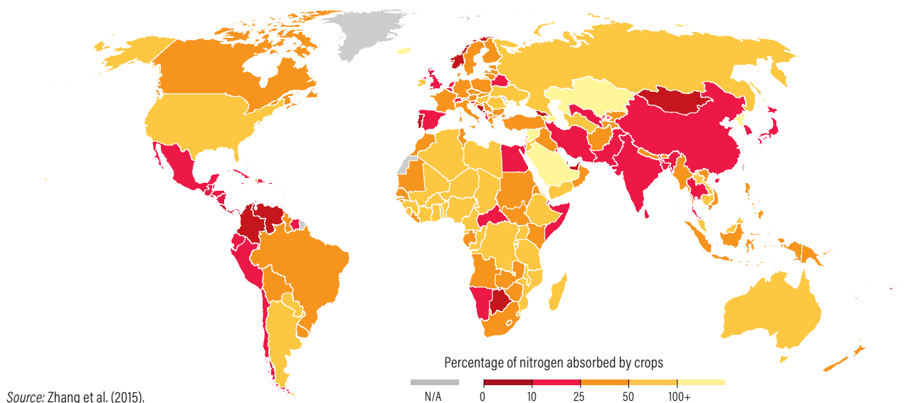
Figure 19 | The percentage of applied nitrogen that is absorbed by crops varies widely across the world
